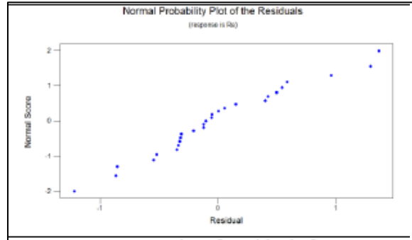
Fig: 4. Normplot of Residuals for MRR
